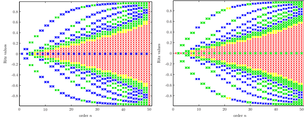
FIG. 5.3. Ritz values of order n = 1, \dots, N for equidistant eigenvalues on [-1, 1] , eigenvectors 1/\sqrt{N} , and poles (\xi, -\xi, \xi, -\xi, \dots) , \xi = 10^{-5} . On the left for N = 50 even, we find for odd n that the Ritz value 0 is not close to any of the eigenvalues (Case 2), and for even n Case 4 occurs. On the right for N = 51 odd, we find for odd n that the Ritz value 0 hits the exceptional eigenvalue 0 (Case 5), and for even n there are two Ritz values not so close to the exceptional eigenvalue 0 (Case 3), that is, there is a delay in the convergence.
