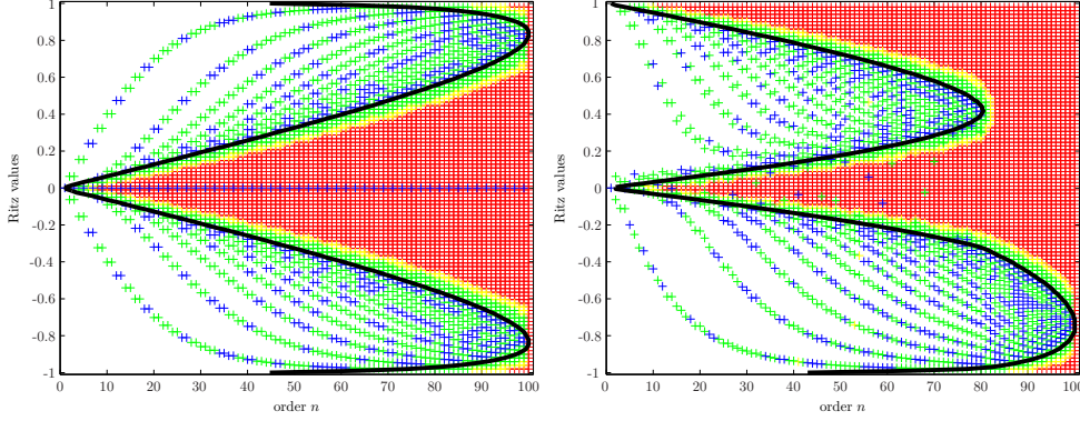
FIG. 4.2. In these figures we plot Ritz values of order n = 1, \dots, N . The colors indicate the distance of a Ritz value to a closest eigenvalue of A_N ( N = 100 ) with equidistant eigenvalues in [-1, 1] . The solid black line is the boundary of \text{supp}(\sigma - \mu) as a function of t = n/N . In the left figure all poles are at 0 and in the right figure the poles are alternating (0, 1, 0, 1, \dots) .
