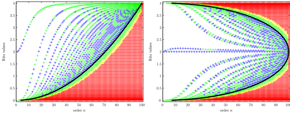
FIG. 4.3. In these figures we plot the Ritz values of order n = 1, \dots, N . The colors indicate the distance of a Ritz value to a closest eigenvalue of A_N ( N = 100 ) with equilibrium-distributed eigenvalues in [0, 4] . The solid black line is the boundary of \text{supp}(\sigma - \mu) as a function of t = n/N . In the left figure the poles are (0, \infty, 0, \infty, \dots) and in the right figure the poles are (0, 4, 0, 4, \dots) .
