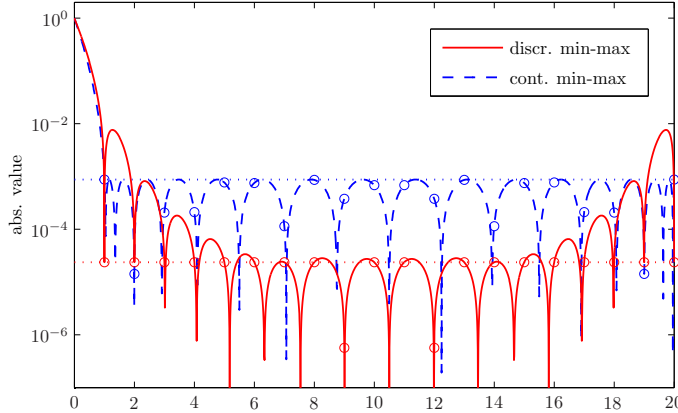
FIG. 2.1. The absolute value of two polynomials of degree 17 taking value 1 at 0. One polynomial (solid red) is minimal on the discrete set \{1, 2, \dots, 20\} , and the other polynomial (dashed blue) is minimal on the interval [1, 20] .
