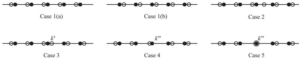
FIG. 5.1. Examples of relative positions of the Ritz values and the eigenvalues in a closed interval J not containing the extremal eigenvalues. The Ritz values are depicted by circles, the eigenvalues are depicted by black dots. The \lambda_{k^*(N)} and \lambda_{k^{**}(N)} indicate the exceptional positions in Proposition 5.3 and in the proof of the lower bound in Theorem 3.1.
