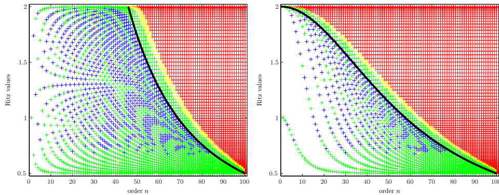
FIG. 4.1. In these figures we plot Ritz values of order n = 1, \dots, N . The colors indicate the distance of a Ritz value to a closest eigenvalue of the Toeplitz matrix A_N from the Kac-Murdock-Szegő example ( N = 100 , q = 1/3 ). The solid black line is the graph of b(t) , t = n/N . In the left figure all poles are in \xi = 10 and in the right figure all poles are in \xi = 2 .
